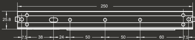
Lock Body Top view
