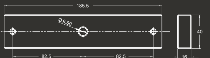
Armature Plate Front view
